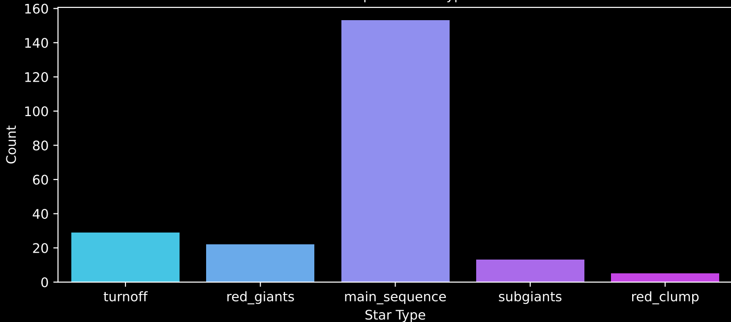
APOGEE DR17 Field: [190-60] Count plot of Star Type
