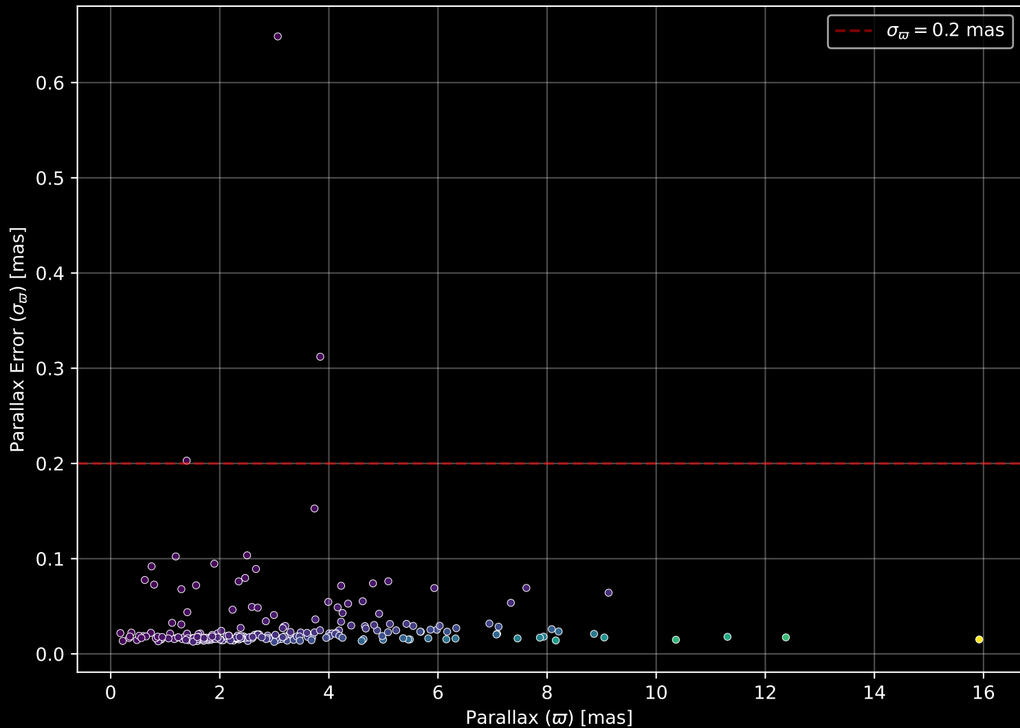
APOGEE DR17 Field: [190-60] Parallax Quality (n= 222)
