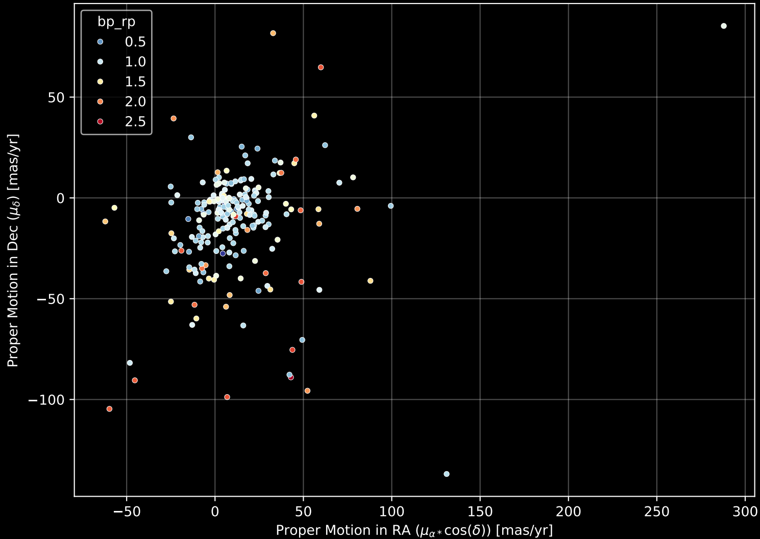
APOGEE DR17 Field: [190-60] Proper Motion Diagram (n= 222)
