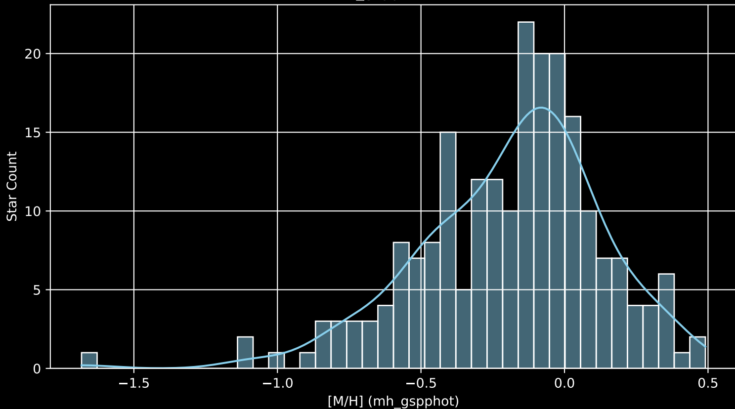
APOGEE DR17 Field: [190-60 [M/H] (mh_gspphot) (n= 217)
