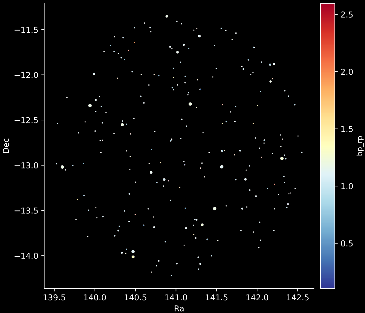
APOGEE DR17 Field: [190-60] Stars: 222
