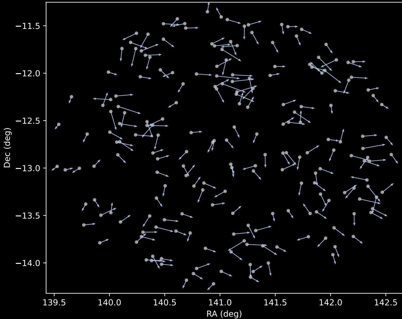
APOGEE DR17 Cluster 1 Proper Motion Vectors (n=204)
