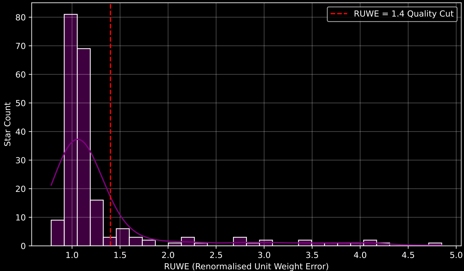
GAPOGEE DR17 Field [190-60] RUWE Distribution (n= 210)
